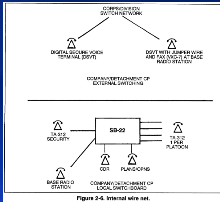
Figure 2-6. Internal wire net.
